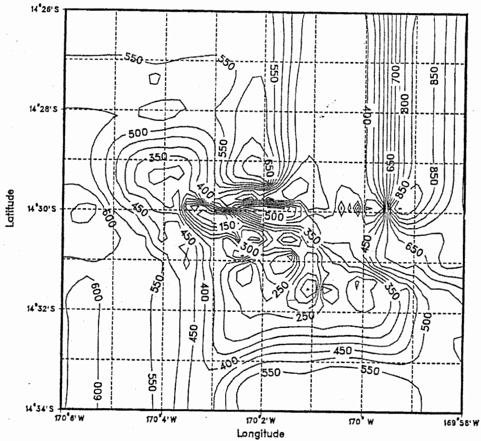
Figure 4.--Bathymetric contours of the Southeast Bank (Bank 3). Note that the contour interval is 94 m (50 fathoms) and 1.0 min of latitude is equal to 1.85 km.
