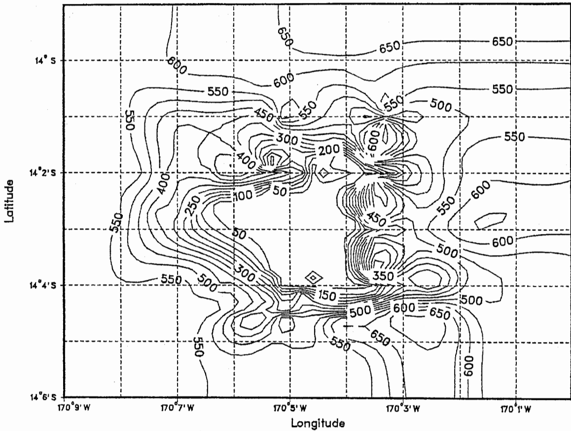
Figure 5.--Bathymetric contours of the Northeast Bank (Bank 4). Note that the contour interval is 94 m (50 fathoms) and 1.0 min of latitude is equal to 1.85 km.
