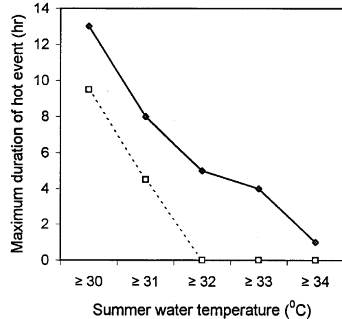
Fig. 4 Mean (above) and maximum (below) duration of summer hot water events in pools A (1998-1999) and B (1999-2000). Frequency of hot events (above) refers to number of days during which a brief period of hot water occurred
